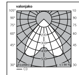
SYLWING SM 2x35W
