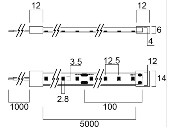
Flex Pro 72W CRI90 IP65
