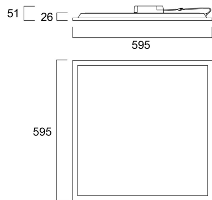
ON/OFF UGR19 mikroprisma
