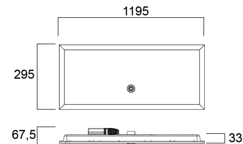
SylSmart Connected mikroprisma
