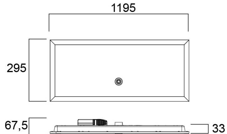
1200x300 mm SylSmart Connected
